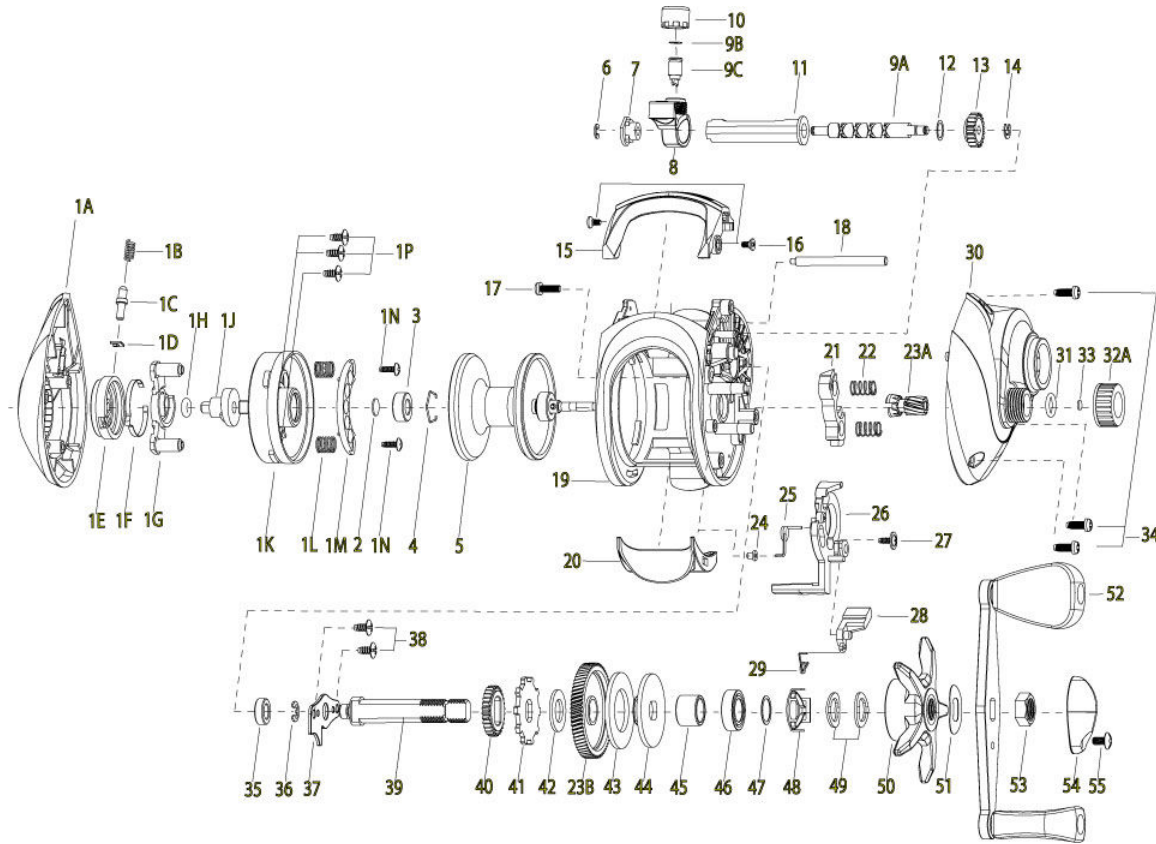
Quantum Ultra UL460CX Baitcast Reel Part List
