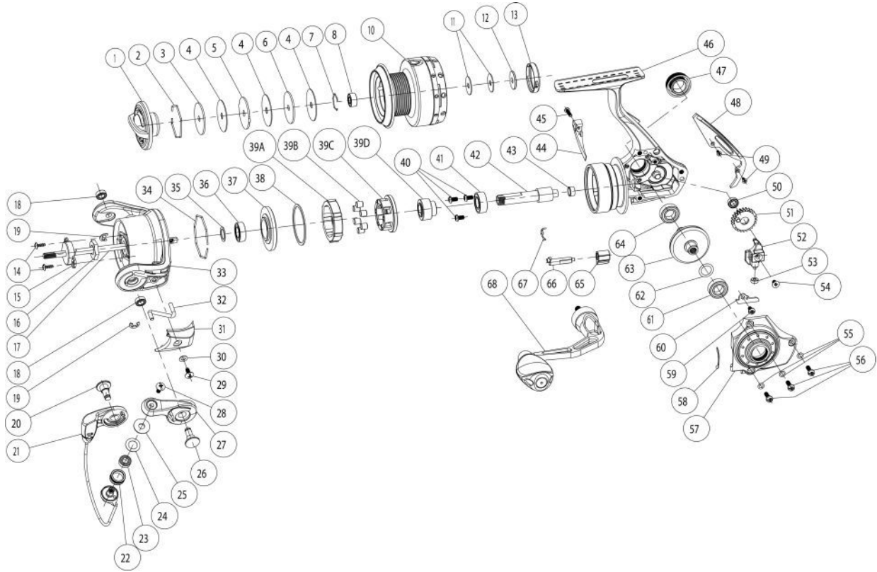
Quantum Tour Edition TE20PTIB Spinning Reel Part List
