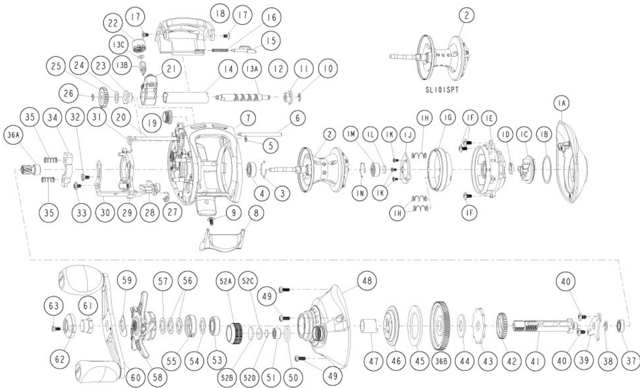
Quantum SL101SPT Bait Cast Reel Part List
