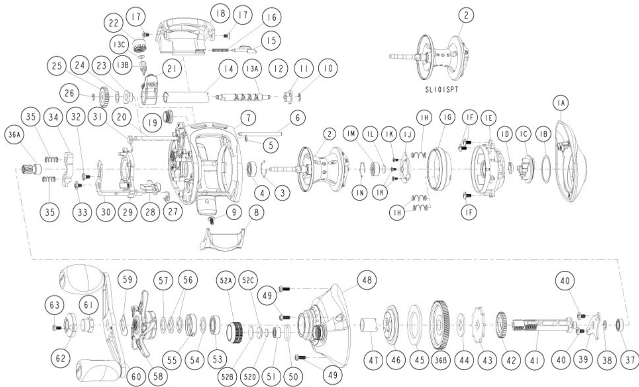
Quantum SL101HPT Bait Cast Reel Part List
