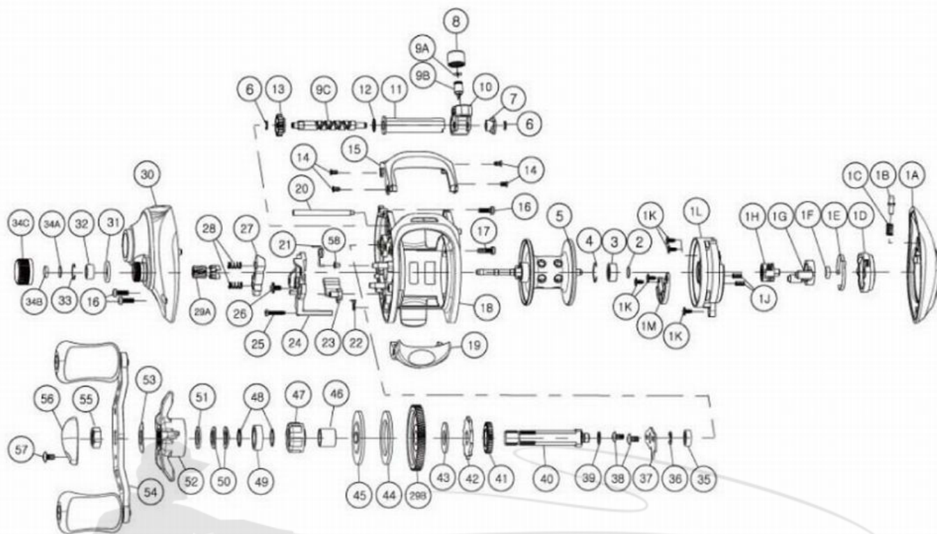
Quantum UL101S Baitcast Reel Part List
