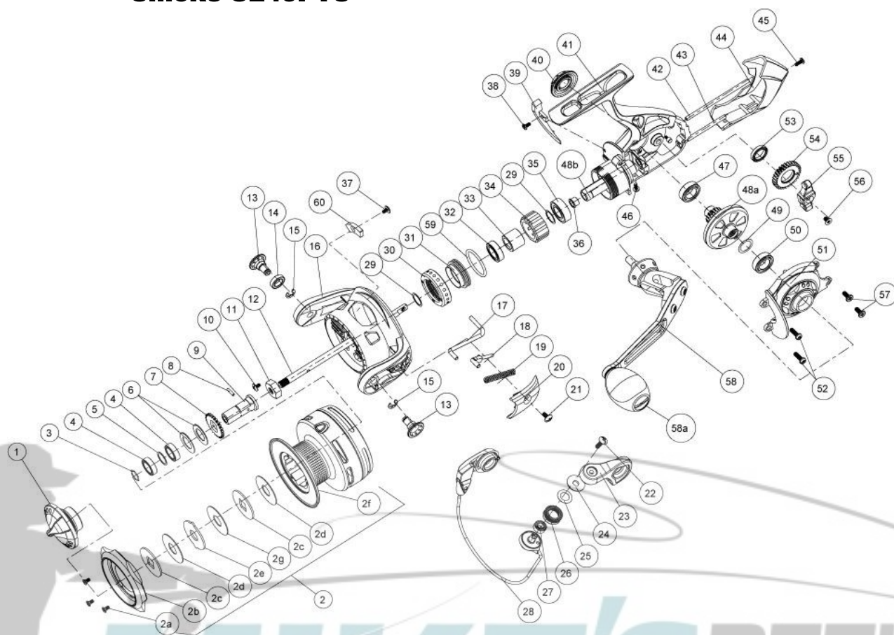
Quantum Smoke SL40PTS Spinning Reel Part List
