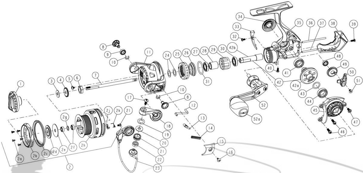
Quantum Smoke SL15PTi Spinning Reel Part List
