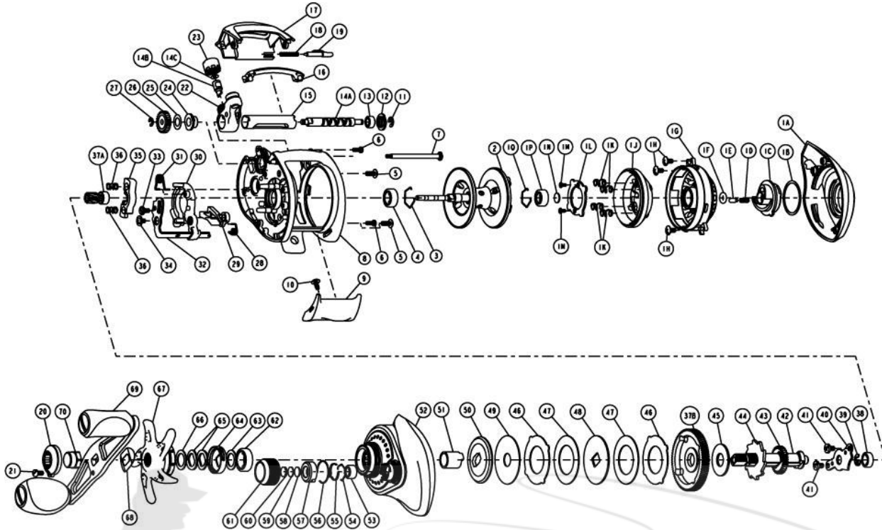
Quantum SL151HPT Bait Cast Reel Part List
