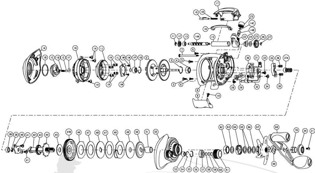
Quantum SL150PPT Bait Cast Reel Part List
