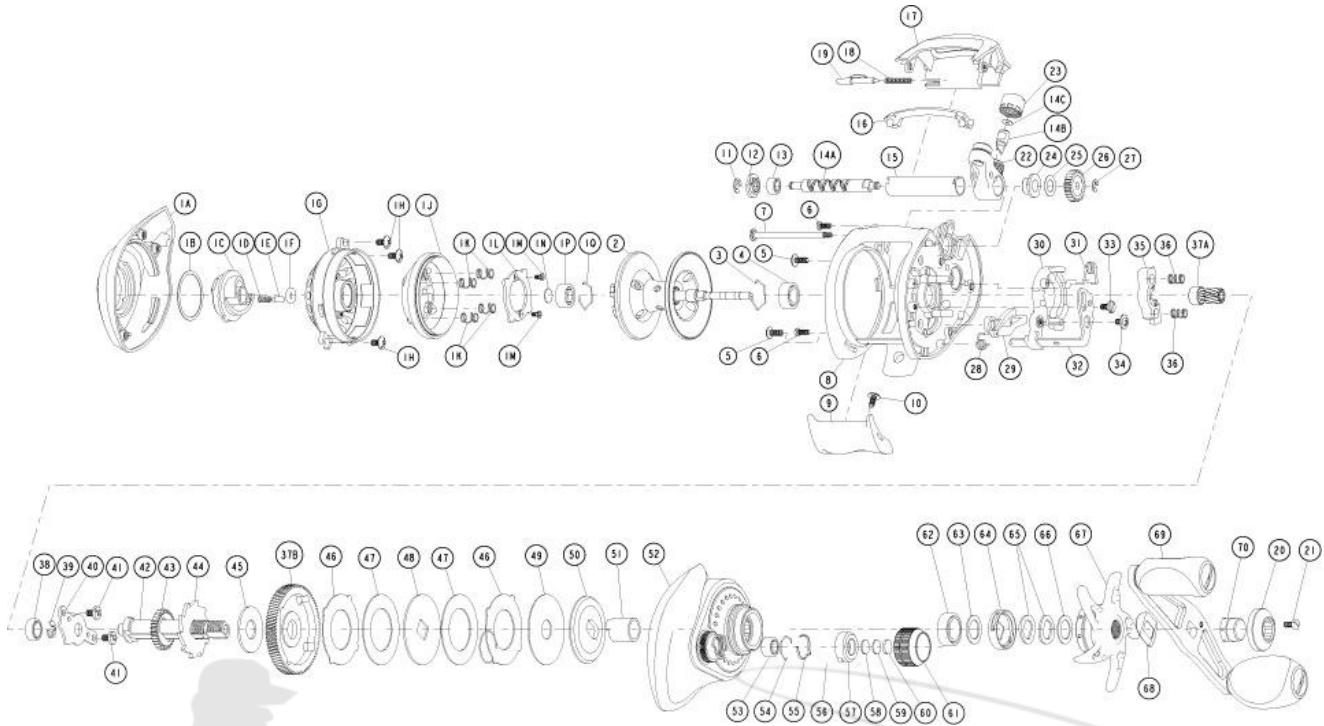
Quantum SL150HPT Bait Cast Reel Part List
