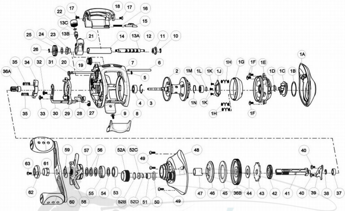
Quantum SL101HPTS Bait Cast Reel Part List
