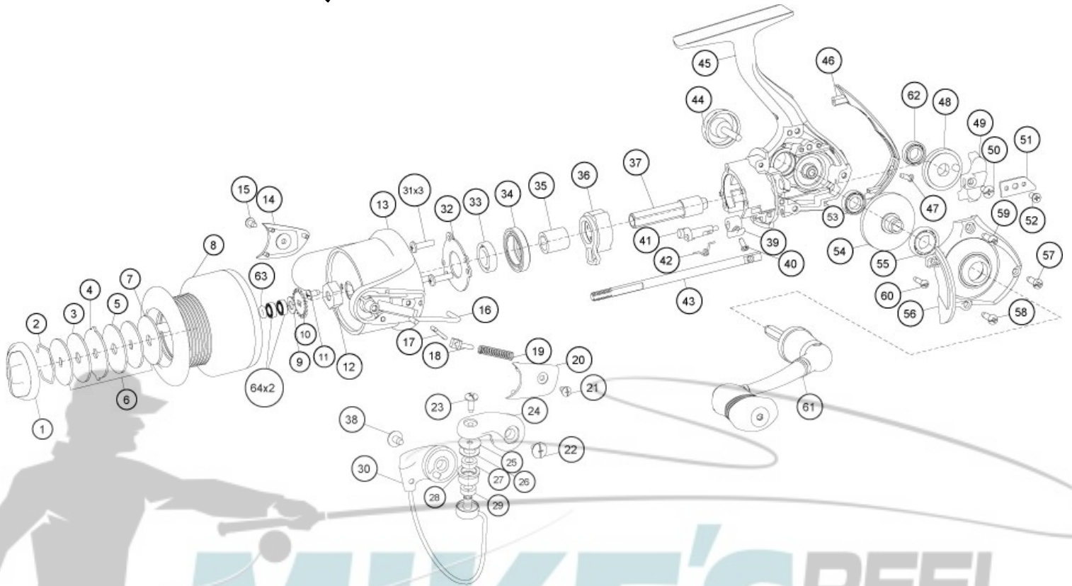
Quantum QV30 Spinning Reel Part List
