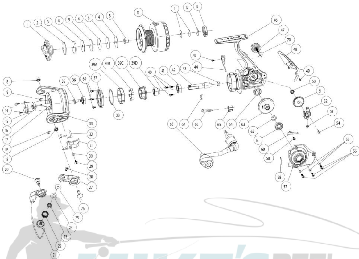
Quantum Kinetic KT40PTIB Spinning Reel Part List
