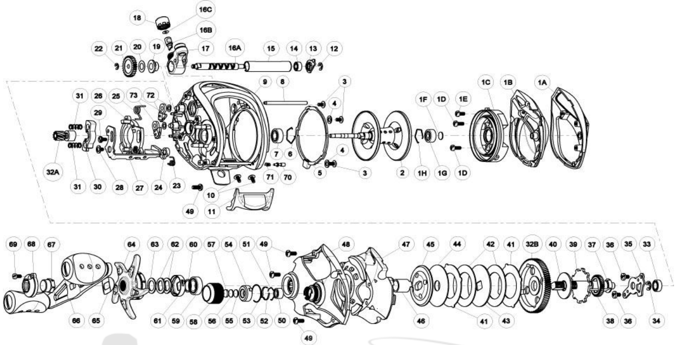
Quantum EX201SPT Bait Cast Reel Part List
