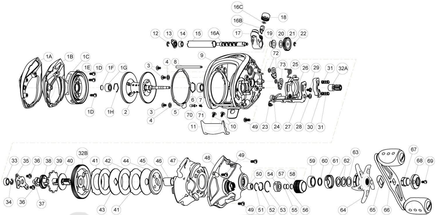
Quantum EX200PPT Bait Cast Reel Part List
