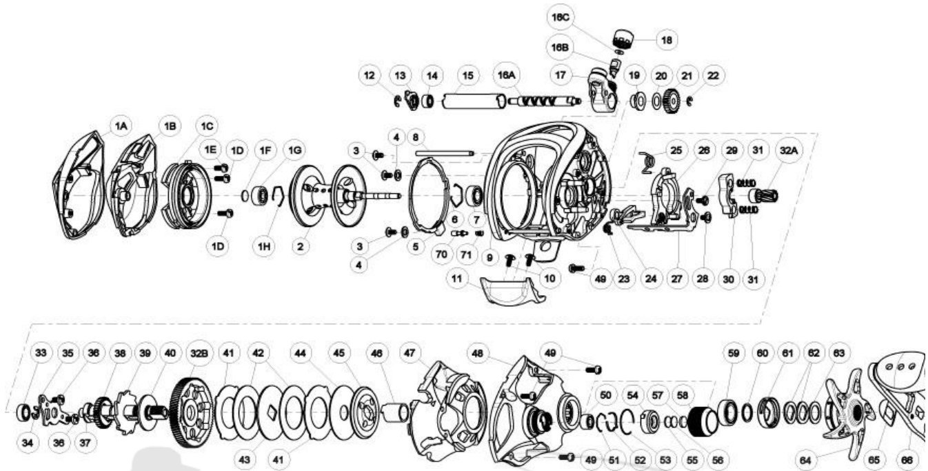
Quantum EX100SPTA Bait Cast Reel Part List
