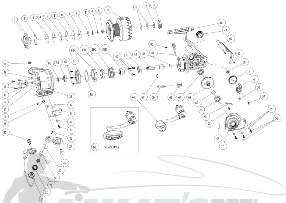
Quantum Energy EI50PTsB Spinning Reel Part List
