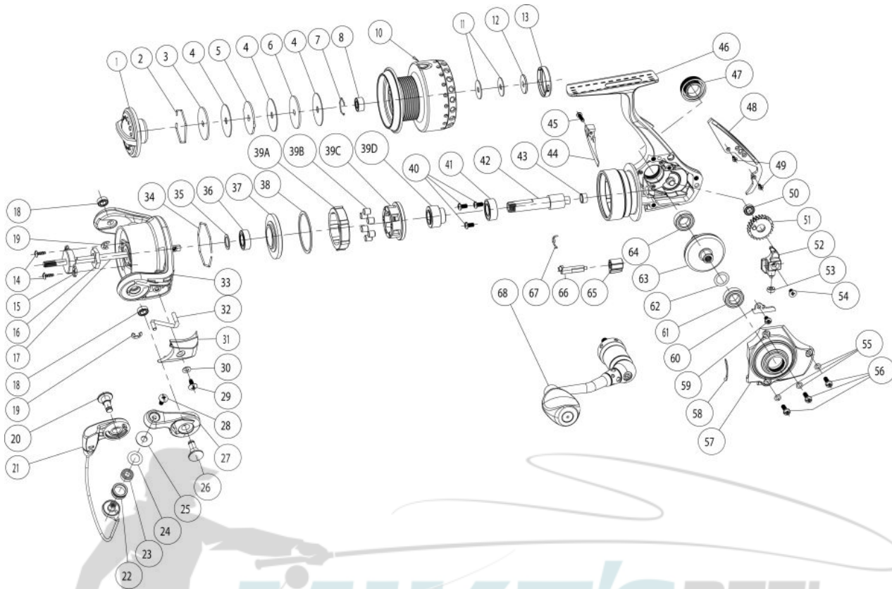
Quantum Energy EI20PTsB Spinning Reel Part List
