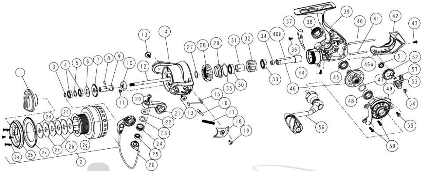
Quantum E30PTiC Spinning Reel Part List
