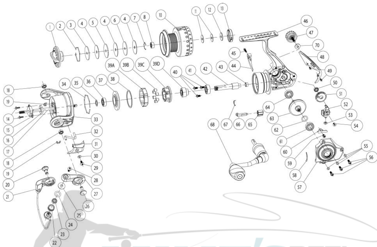
Quantum Energy CT20PTIB Spinning Reel Part List
