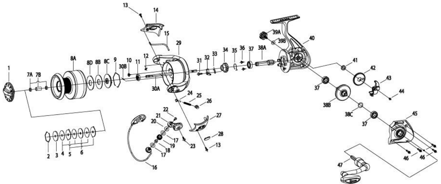
Quantum BLUE RUNNER BR70F Part List
