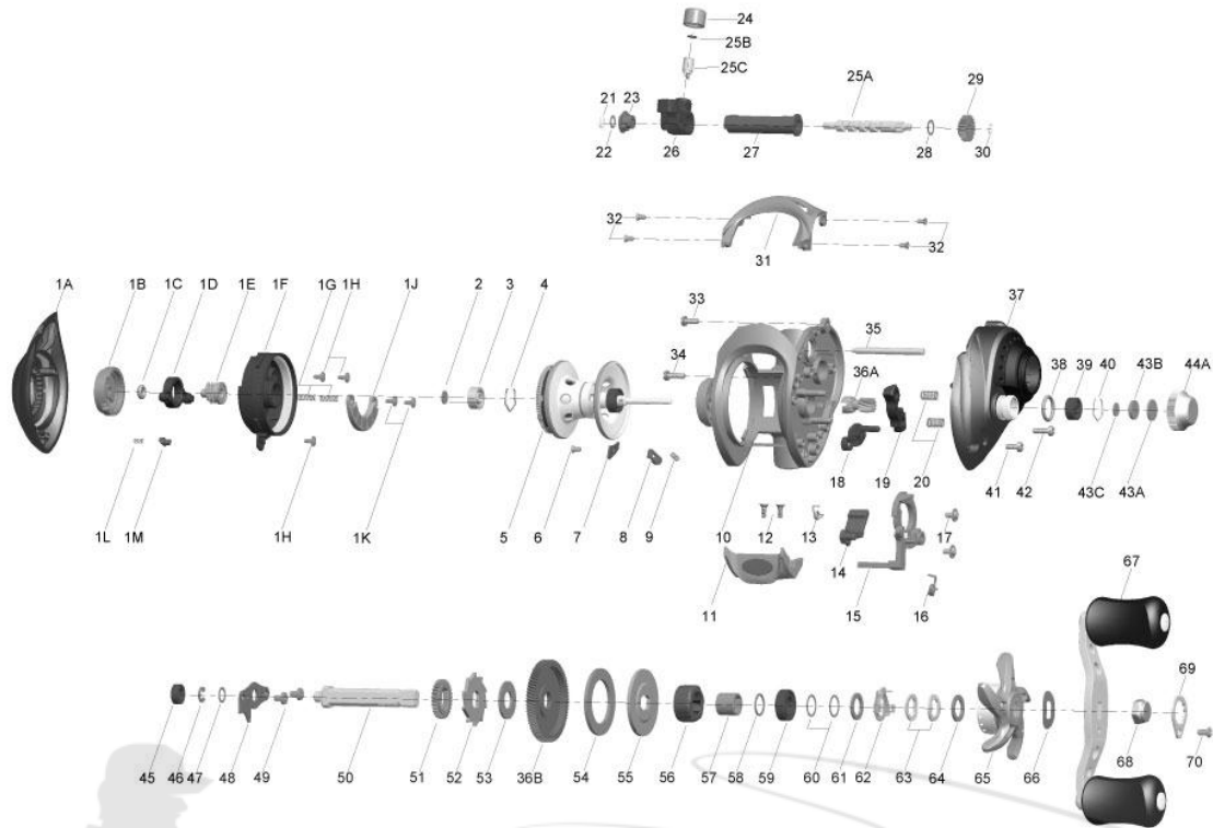
Quantum AN100H Bait Cast Reel Part List
