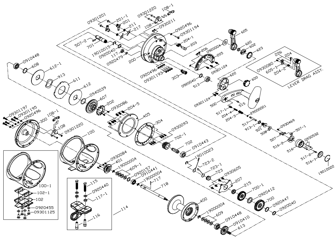
Makaira 50-II PARTS LIST
