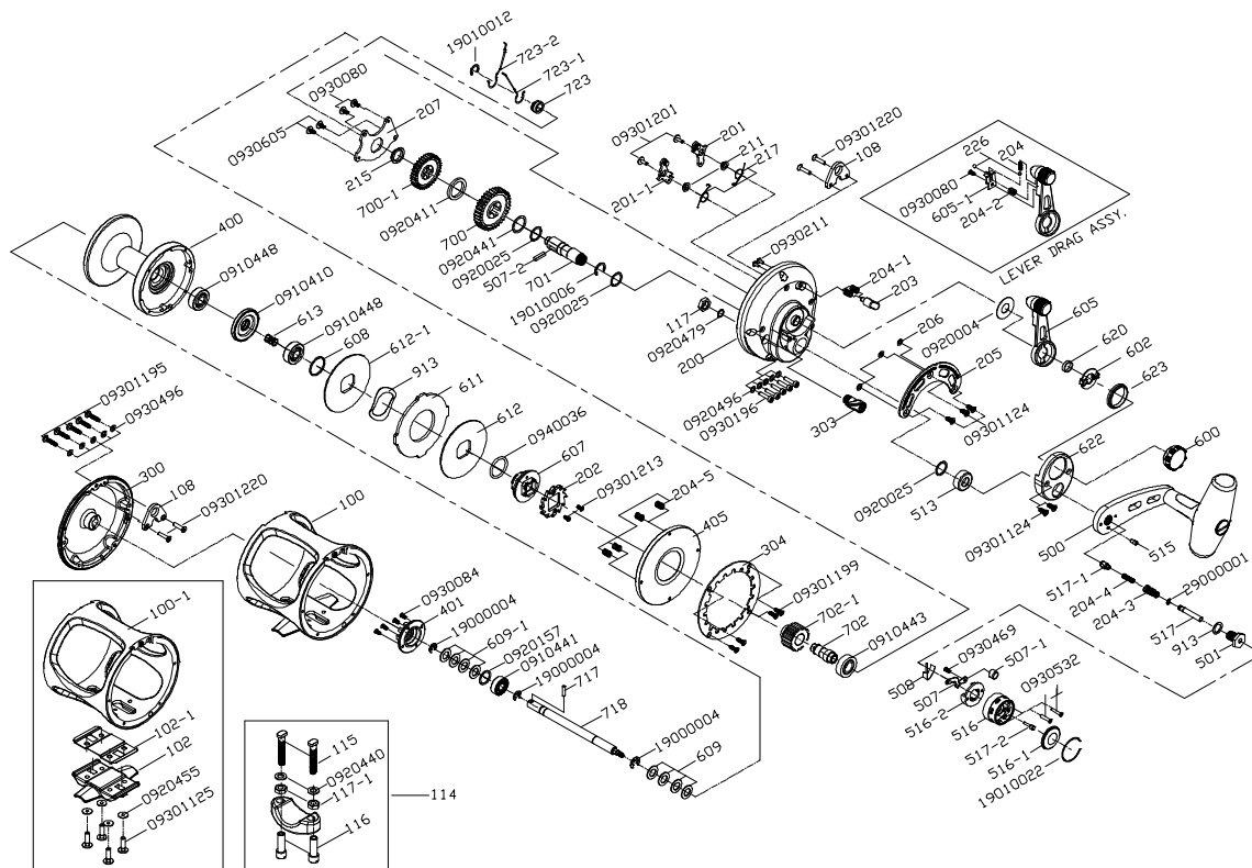
Makaira 30-II PARTS LIST
