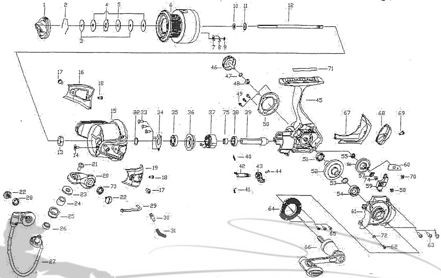
PARTS LIST OF MTX308XE/308XGE/300XE/300XGE
