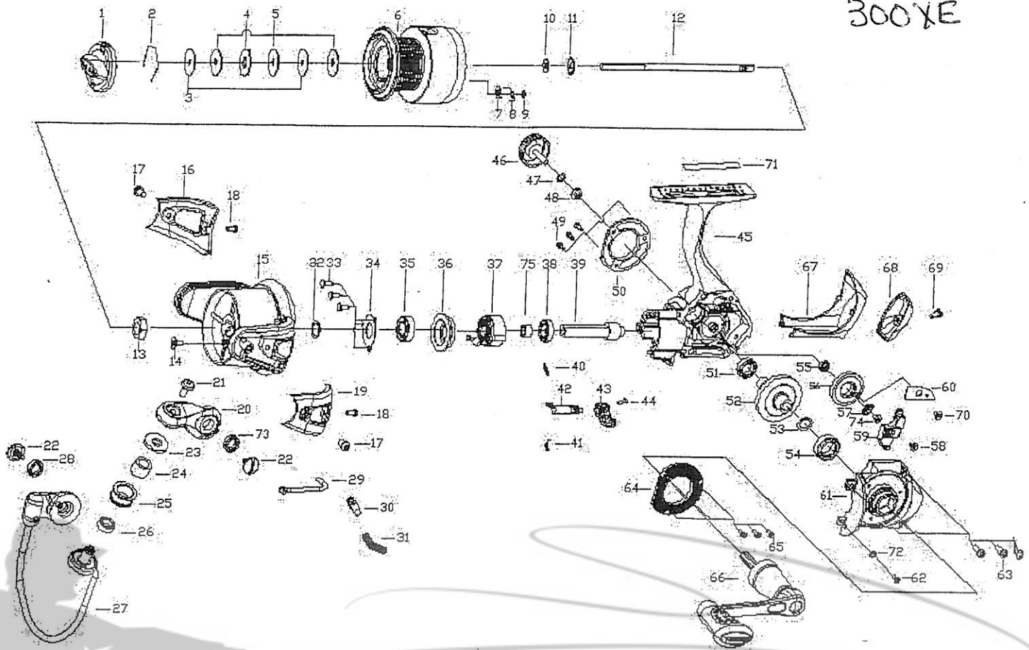
PARTS LIST OF MTX308XE/308XGE/300XE/300XGE
