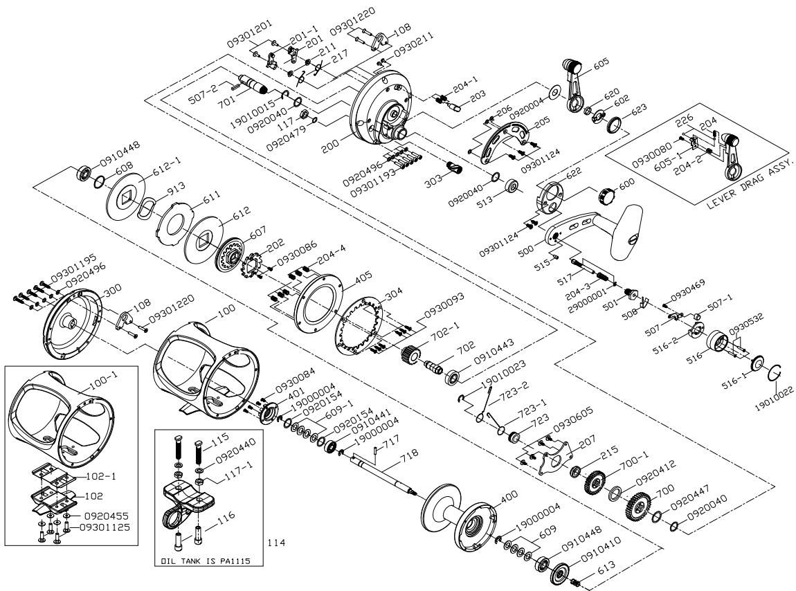
Makaira 50W-II PARTS LIST
