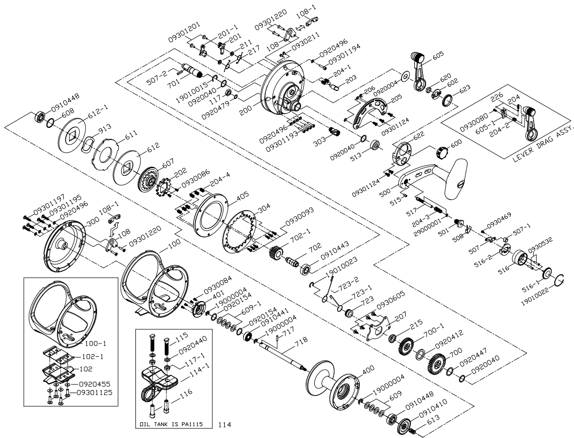
Makaira 50-II PARTS LIST
