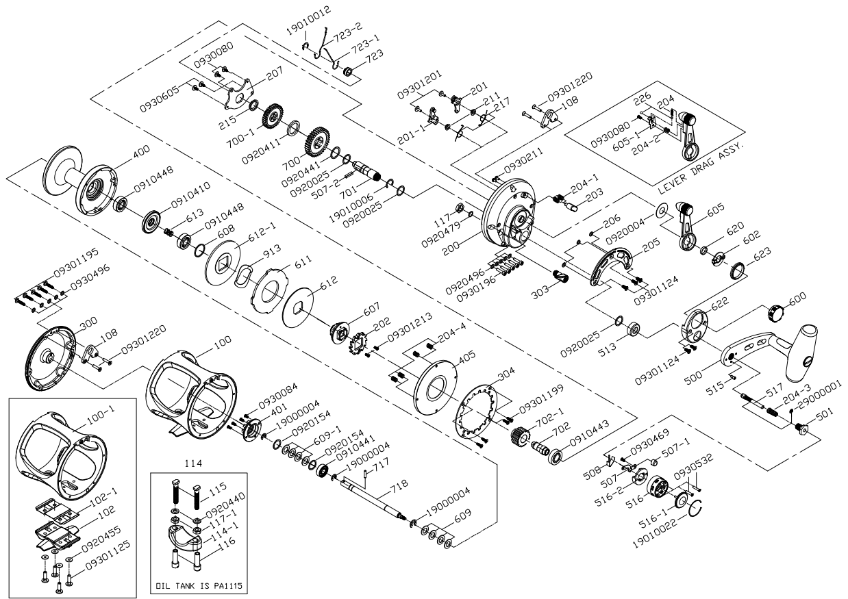
Makaira 30-II PARTS LIST
