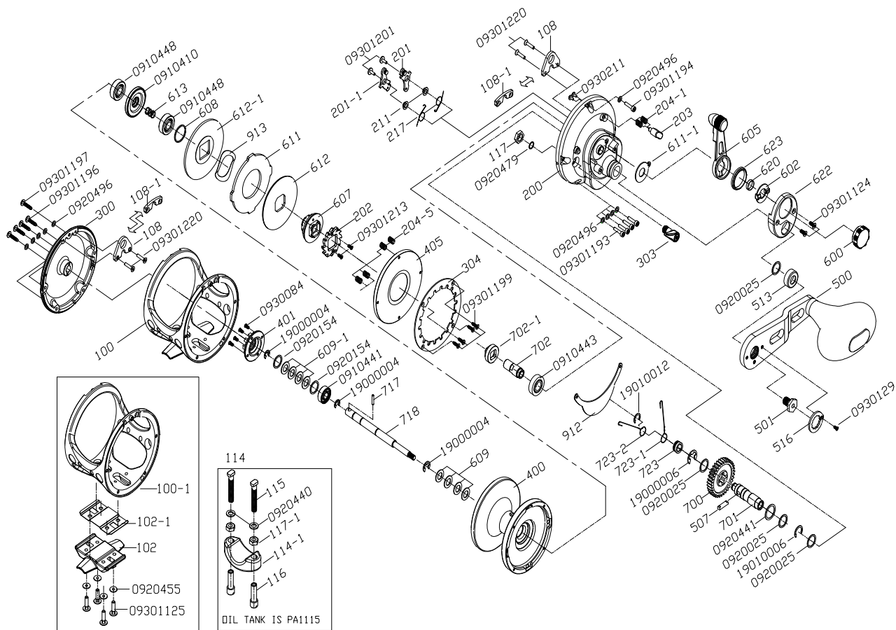
CLD-20S PARTS LIST
