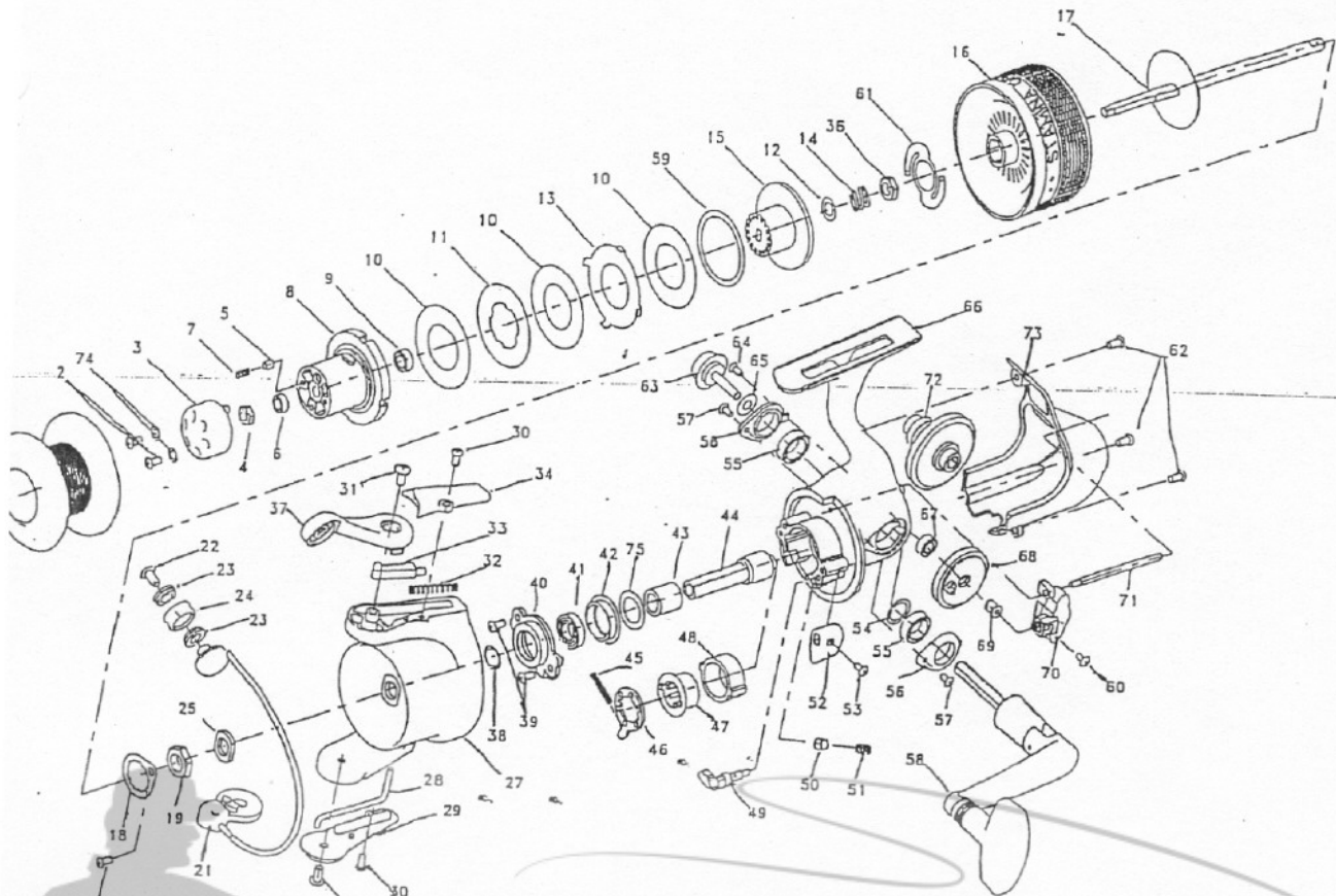
ABU GARCIA CARDINAL 704/774 PARTS LIST
