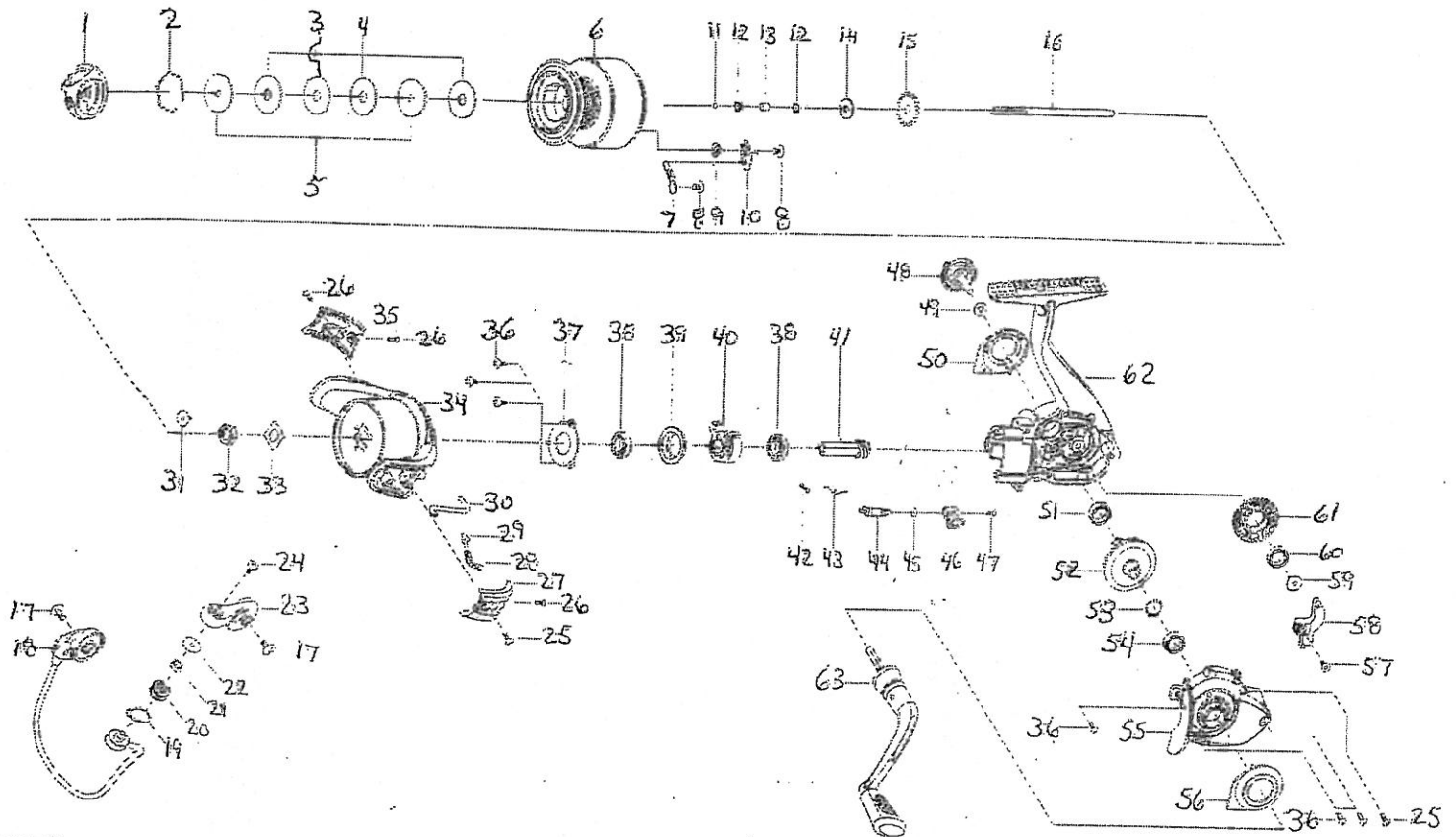
PARTS LIST OF AVOCET II G4000FD
