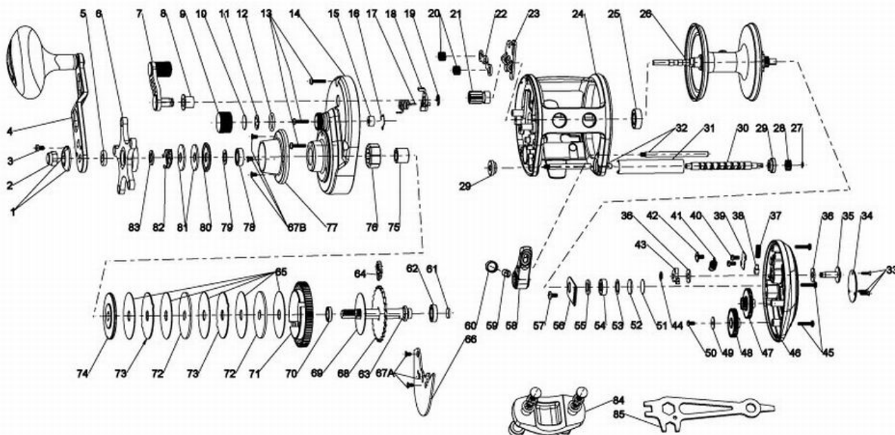
Fin-Nor Offshore Level-Wind OFL20 Reel Part List
